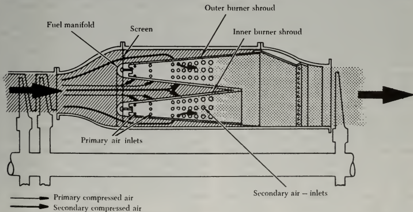
FIGURE 1-46. Components and airflow of a double-annular chamber.
